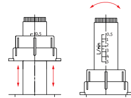
Adjusting the flow meter + lift lock-ring
